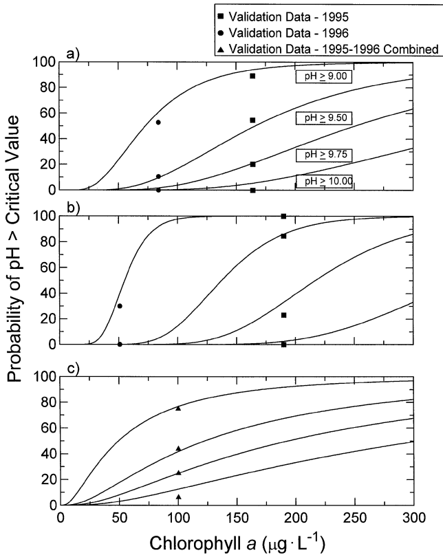
Fig. 3. Probability of exceeding four critical pH levels computed from the regression-based probability models developed for Upper Klamath and Agency lakes. Probability curves are computed from eq. 5 with input parameters from Table 1 (model subset descriptions for a , b , and c are the same as for Fig. 2). Symbols represent observed exceedence frequencies from the independent model validation data set and are plotted against mean Chl (see text for detailed explanation).
